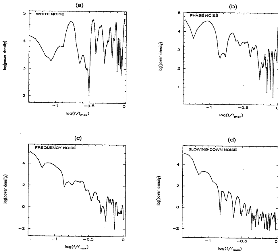
Figure 5. Power density spectra of the non-uniformly sampled time sequences shown in Fig. 3. The spectra were obtained using the technique based on 'CLEAN'.
