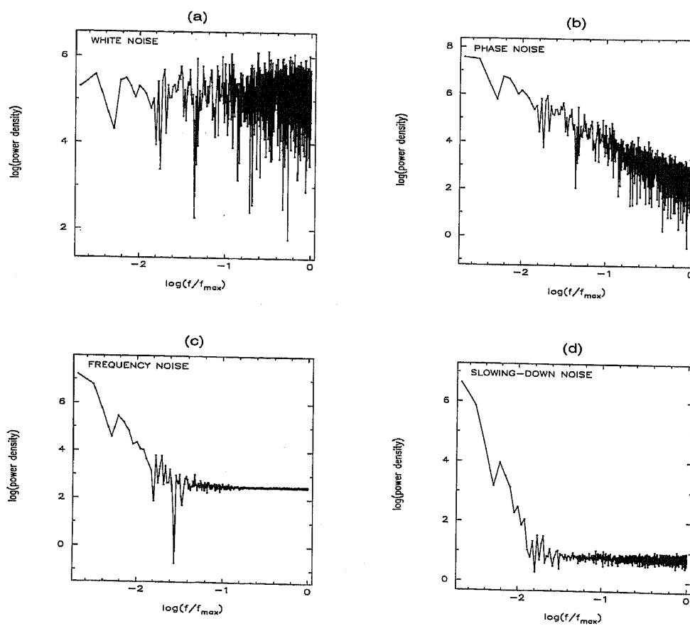
Figure 2. Power density spectra of the simulations shown in Fig. 1. The plots show log(power density) as a function of \log(f/f_{max}) in the four cases.
