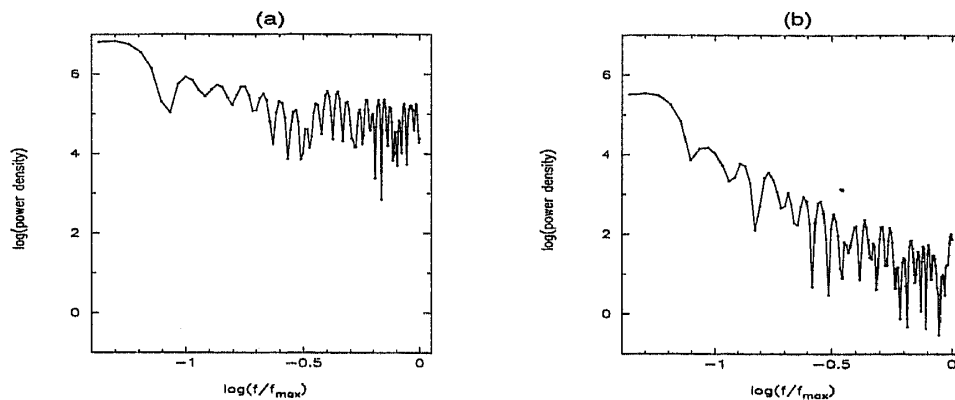
Figure 6. The power density spectrum estimated from the phase residuals for PSR 1641–45 using: (a) conventional discrete Fourier transform methods, and (b) the 'CLEAN' technique.
