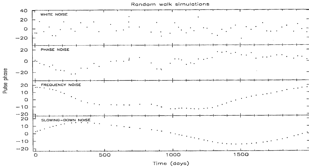
Figure 3. Simulations of white noise, phase noise, frequency noise and slowing-down noise, sampled according to the observation epochs for PSR 1641-45.
