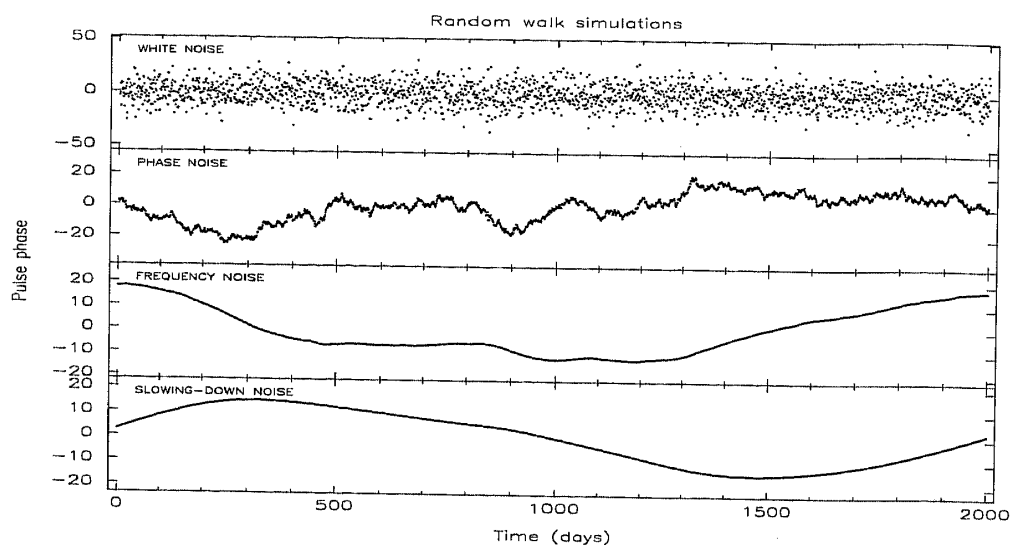
Figure 1. Uniformly sampled time sequences which simulate white noise (WN), phase noise (PN), frequency noise (FN) and slowing-down noise (SN) respectively, with 0.1% of white noise added to the sequences for PN, FN and SN.
