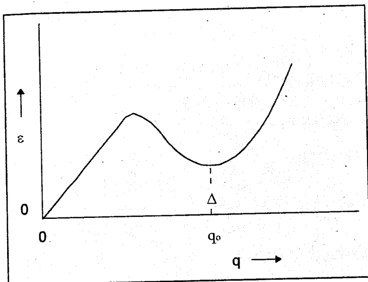
Figure 1. Dispersion curve in LHe II.
