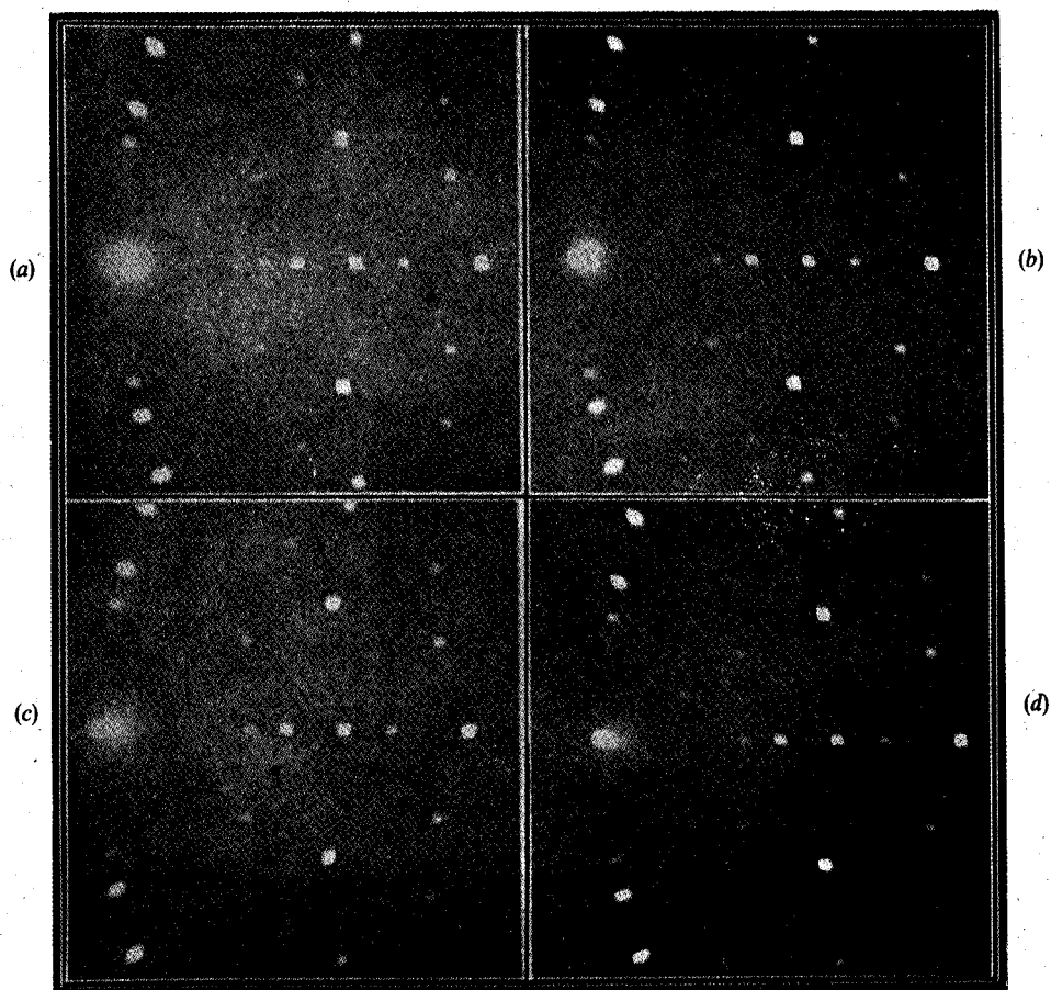
Figure 1. Exhibiting the dynamic reflections by the (400) planes at the left.
