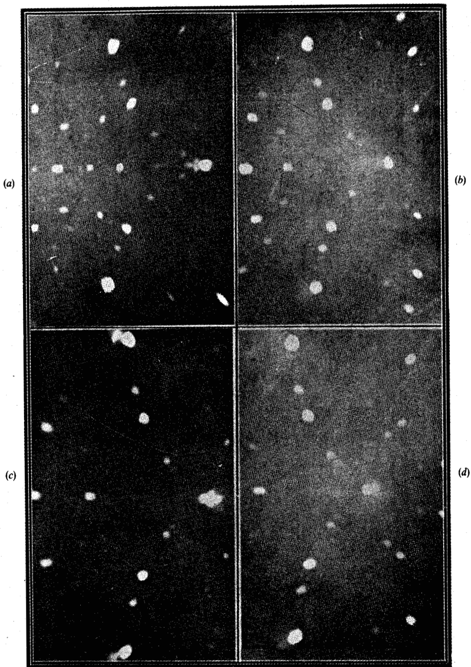
Figure 1. Exhibiting the dynamic reflections by the (111) planes of tetrahedral diamond on the left and their absence with octahedral diamond on the right.
