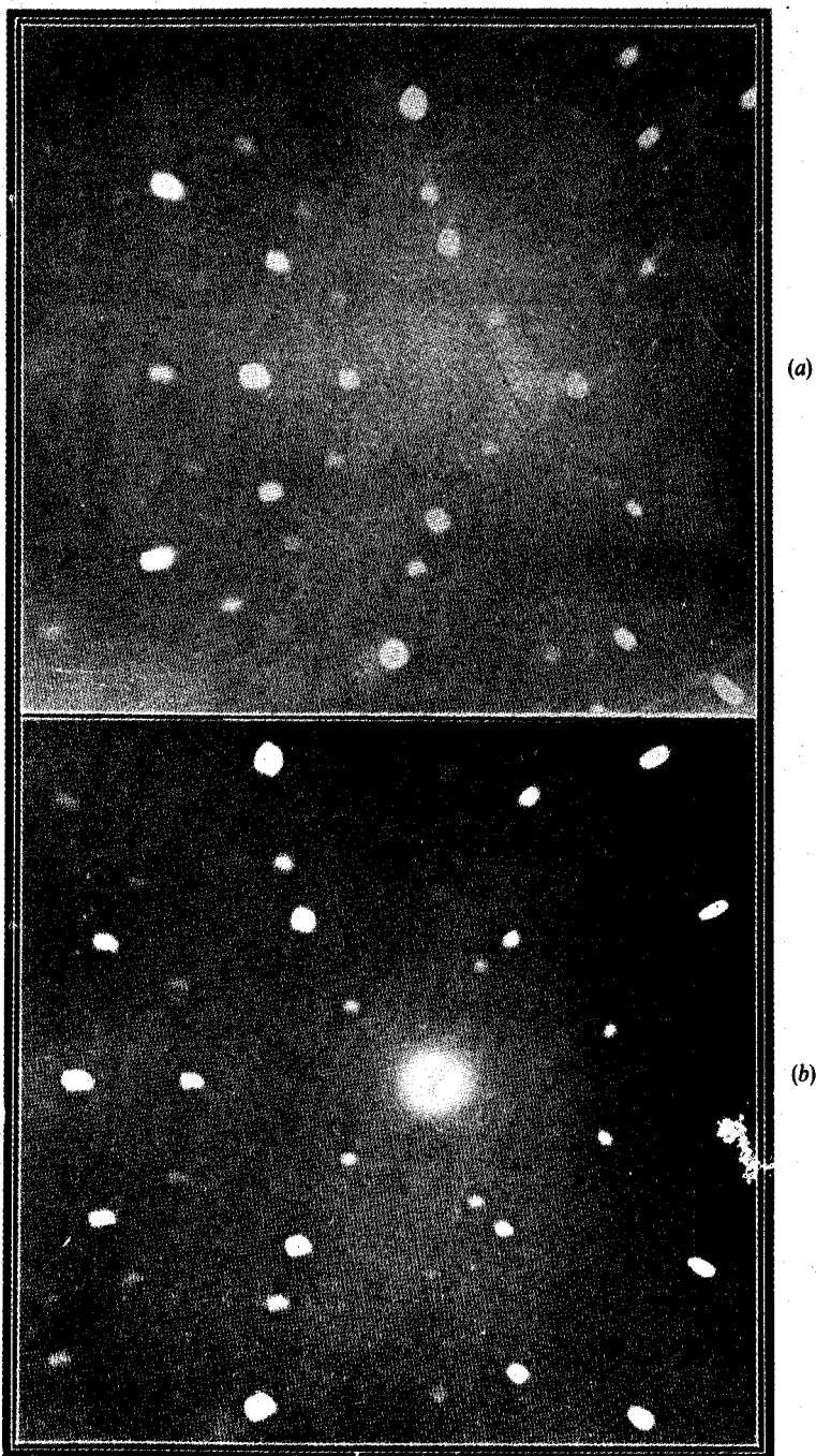
Figure 1. Laue patterns of octahedral diamond showing intense reflection by the (111) planes at different settings.
