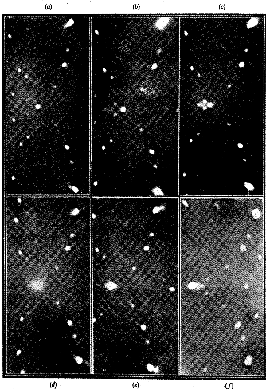
Figure 1. Exhibiting the dynamic reflections by the (111) planes of various settings.
