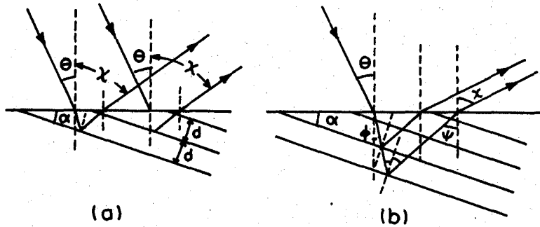
Figure 3. Identity of direction of iridescent reflection with diffraction spectrum.
