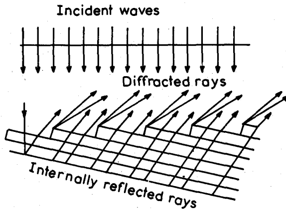
Figure 19. Asymmetrical diffraction of internally reflected rays on emergence.
