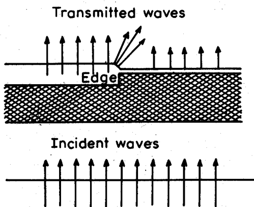
Figure 18. Asymmetrical diffraction by laminar edge.
