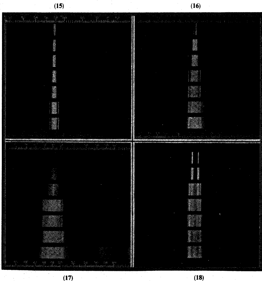
Figures 15-18. Reflection spectra of iridescent crystals.
