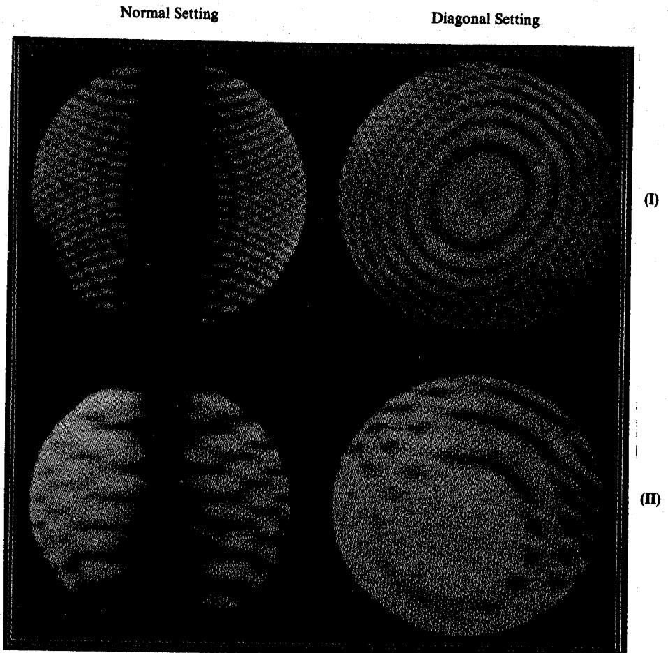
Symmetric conoscopic patterns.
