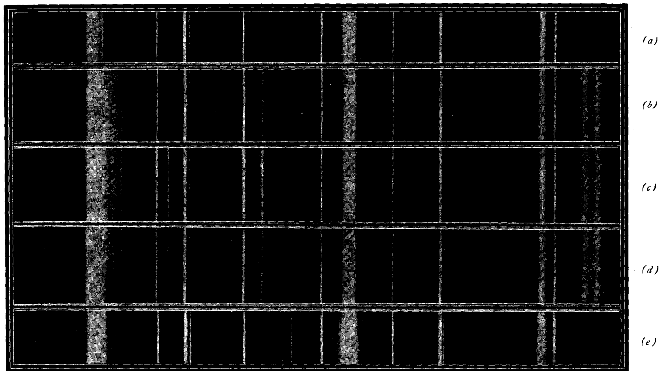
FIG. 1. The Raman spectra of various forms of gypsum: (b) Selqite; (c) Fascicular gypsum; (d) Alabaster. (a) and (e) Spectrum of the mercury arc.
