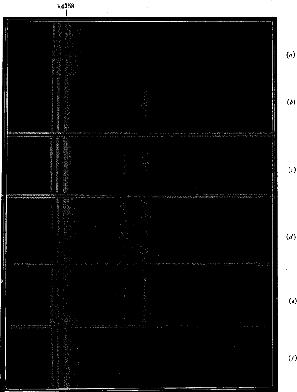
(a) Spectrum of the mercury arc; (b) and (c) Raman spectrum of rutile at room temperature for two different orientations of the crystal; (d) Heavily exposed Raman spectrum of rutile at room temperature; (e) The spectrum of the rutile at liquid air temperature; (f) Spectrum of the mercury arc.
