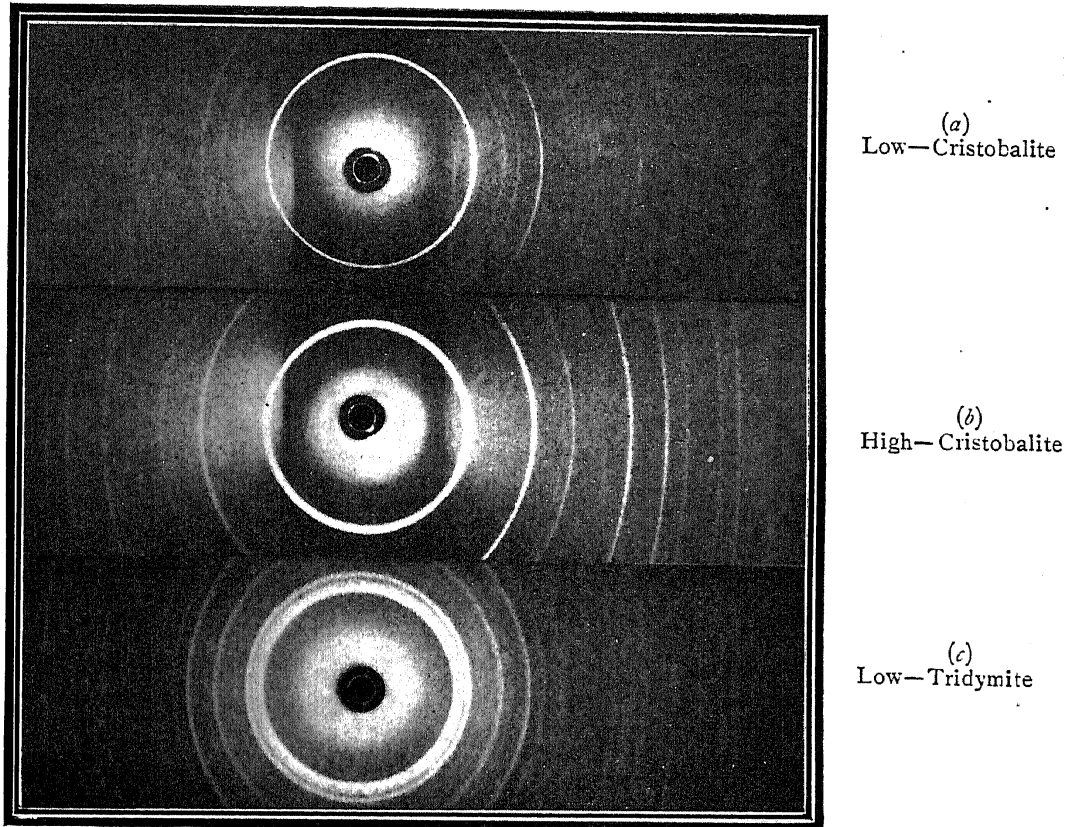
FIG. 2. X-Ray Diffraction Patterns
