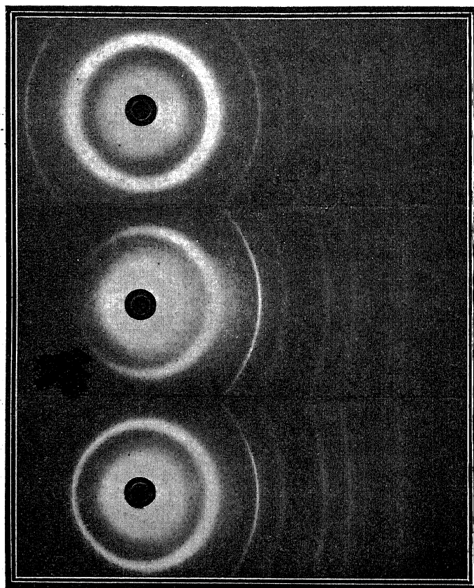
FIG. 3. X-Ray Diffraction Patterns
