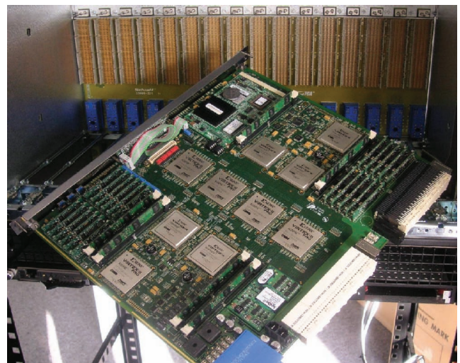
Figure 8. The CABB DSP board.
