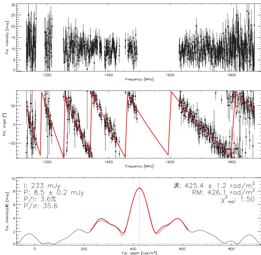
Figure 30. The polarization properties of an extragalactic source on a line of sight close to the Galactic supershell GSH287+04–17 [source coordinates: \alpha, \delta(\text{J2000}) = 10^{\text{h}} 48^{\text{m}} 07^{\text{s}}.653, -53^{\circ} 13' 21''.38 ]. The top and middle panels show the polarized intensity and polarization angle as a function of frequency, which were derived from the observations. The red line in the middle panel indicates the best-fitting \text{RM} = 426 \text{ rad m}^{-2} (the fit has a reduced \chi^2 of 1.5). The bottom panel shows how much power (polarized intensity) is contributed by each Faraday depth. In this case 8.5 mJy is generated at a Faraday depth of 425 \text{ rad m}^{-2} , which matches the average polarized intensity from the top panel and the best-fitting RM from the middle panel well. The solid red line indicates the profile that can be expected from the RM synthesis on the basis of the frequency coverage of the data. The bottom panel illustrates the strength of the RM synthesis: although polarized intensity is detected in each channel at about the 2\sigma level (top panel), combining all frequency channels, which is possible with RM synthesis, gives a detection with a combined polarized signal-to-noise ratio level of 36\sigma (bottom panel; the noise level in the bottom panel is about 0.2 mJy).
