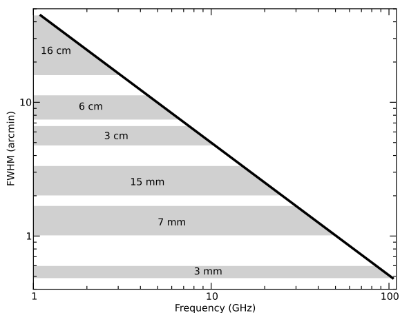
Figure 4. ATCA primary beam FWHM as a function of frequency; values were computed with the MIRIAD task PBPLLOT. The currently available frequency coverage across all ATCA bands from 1.1 to 105 GHz range is indicated by the grey-shaded bands (see also the linear display of the ATCA frequency coverage in Fig. 3).
