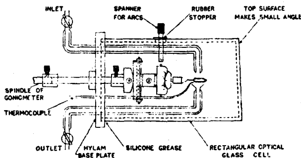
FIG. 2. Low and high temperature attachment to the optical goniometer.
