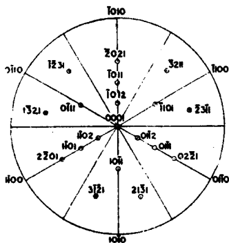
FIG. 3. Stereographic projection of anhydrous lithium nitrate.
