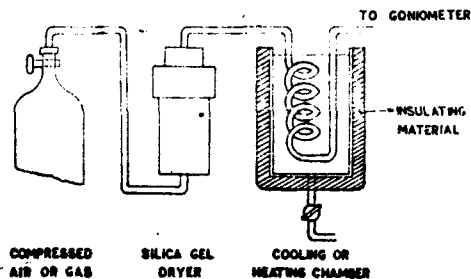
FIG. 1. Device for obtaining dehydrated air (or gas) at different temperatures.
