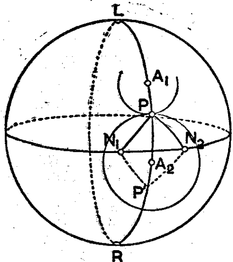
FIG. 4. Location of P by measuring two transmitted intensities.
