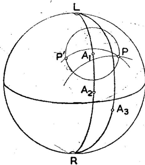
FIG. 3. Location of P by measuring distance of P from any three points A_1 , A_2 and A_3 whose positions are known. For the unique determination of P the three points should not lie on the same great circle.
