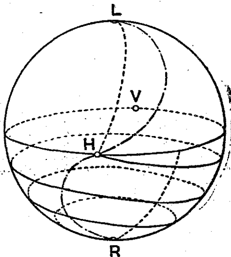
FIG. 7. Scanning the Poincaré sphere along an oblique path. — Path traced by rotating elliptic analyser; both the elements rotating at nearly but not exactly the same speed. - - - Path traced by the combination of a rotating \lambda/4 plate and a stationary linear element. - · - Path of a combination of a fast rotating linear analyser plus a very slow rotating quarter-wave plate.
