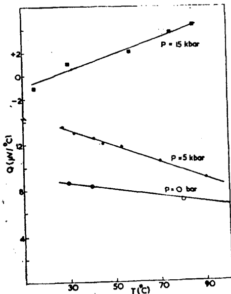
Figure 3. Variation of the thermo-power of cerium with temperature in the \gamma and \alpha -phases.
