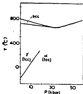
Figure 1. Phase diagram of cerium (Jayaraman 1965).
