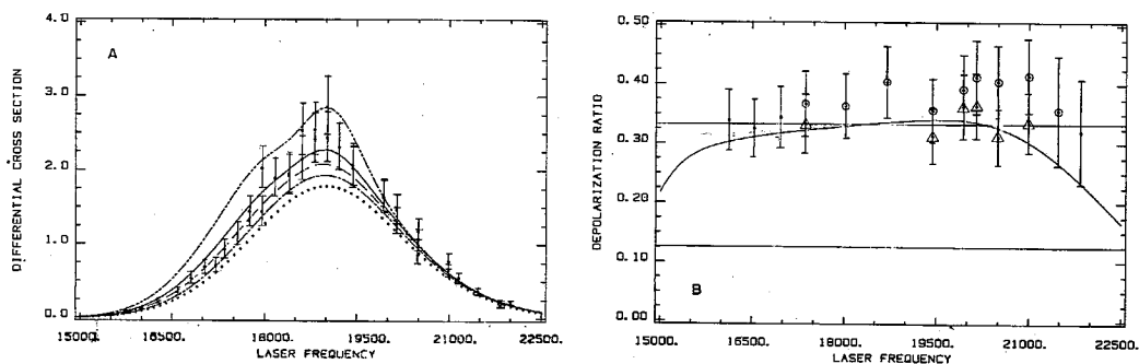
FIG. 8. The calculated and experimental REPs for the first overtone of I_2 in hexane. The error bars are drawn to \pm 15\% . The parameters are the same as in fig. 7 except that the ----- curve was calculated with \Gamma = 10\text{ cm}^{-1} .
