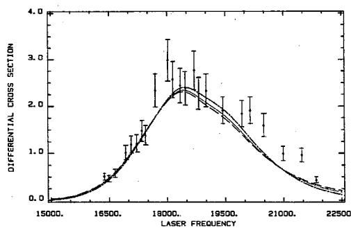
FIG. 10. The calculated and experimental REPs of the I_2 fundamental in perfluorohexane. The error bars are drawn to \pm 10\% . The curves were all calculated with \Gamma = 15 \text{ cm}^{-1} . The dashed line was calculated with the D state contribution with |\mu_{XD}|^2 = 40 D^2 , the solid line was calculated with |\mu_{XD}|^2 = 25 D^2 , and the dot-dashed line was calculated with no D state contribution.
