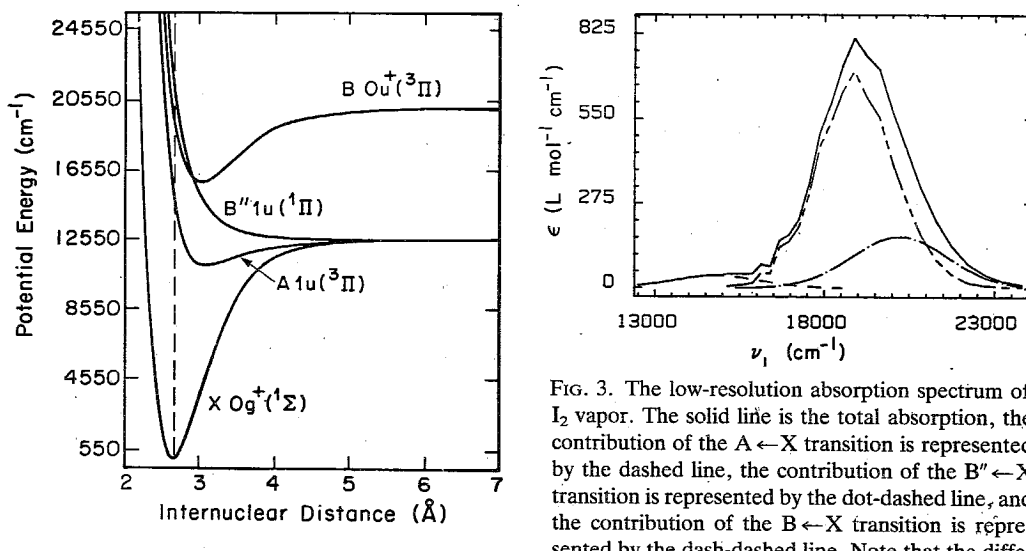
FIG. 2. Potential energy curves for the electronic states of I_2 that contribute to the visible absorption spectrum. The dashed line at 2.67\text{ Å} represents the equilibrium internuclear distance for ground state I_2 (redrawn from ref. 6).
