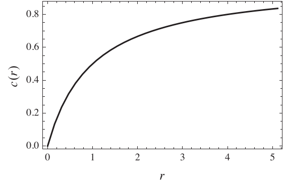
FIG. 3. Proportionality coefficient c(r) between the minimum a^* of I_r(a) and the resetting position x_r . The parameters are \gamma = 1 and \sigma = 1 .
