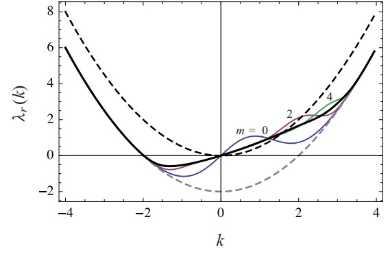
FIG. 1. (Color online) Dominant pole of \tilde{G}_r(x, k, s) for increasing truncation orders: m = 0 (blue), m = 2 (purple), and m = 4 (green). The black curve shows the convex \lambda_r(k) obtained for m \geq 6 , the dashed black curve the nonreset \lambda_0(k) , and the dashed gray curve the tail approximation of \lambda_r(k) shown in Eq. (35). The parameters are x_r = 1 , r = 2 , \gamma = 1 , and \sigma = 1 .
