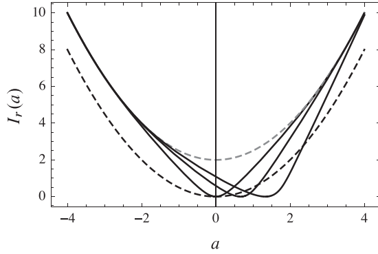
FIG. 2. Black curves represent I_r(a) for x_r = 0, 1, 2 (from left to right). The first two curves were obtained for m = 10 , while the last for x_r = 2 was obtained for m = 20 . The dashed black curve shows the nonreset rate function I_0(a) and the dashed gray curve the tail approximation of I_r(a) shown in Eq. (36). The parameters are r = 2 , \gamma = 1 , and \sigma = 1 .
