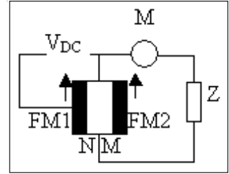
Figure 6. A normal metal is sandwiched between two ferromagnetic metals. A non-equilibrium polarization is induced into NM from FM1 on the left. One will measure a voltage or current on the meter M between NM and FM2 on the right.
