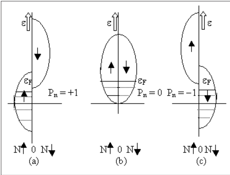
Figure 3. In diagram (a) no energy level for down-spin is occupied as the levels are above the Fermi level; in (b) both up-spin and down-spin levels are occupied by equal number of electrons; in (c) no up-spin level is occupied since all up-spin levels are above the Fermi level.
